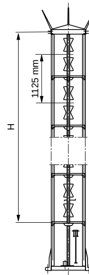
Superturnstile antenna mounted in G.R.P. cylinder with 0.75 m diameter
