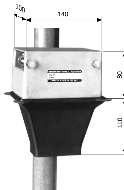
Example 4-way antenna splitter
