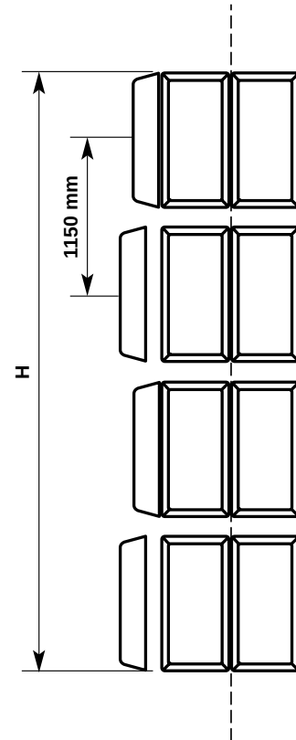
Top view
