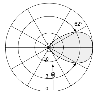
Radiation Patterns (at mid-band)
