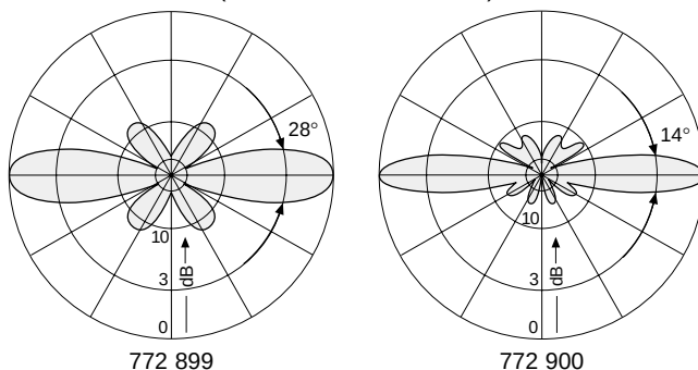
Vertical Radiation Patterns (at mid-band, beamtilt \approx 1^\circ )
