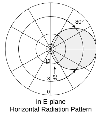
Radiation Patterns (at mid-band)
