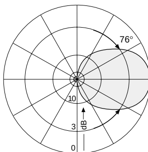
Radiation Patterns (at mid-band)
