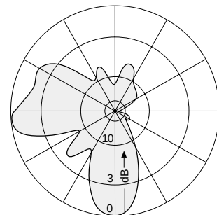
Horizontal Radiation Pattern of the antenna arrangement see above
