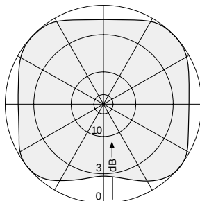
Typical horizontal radiation pattern (at mid-band)
